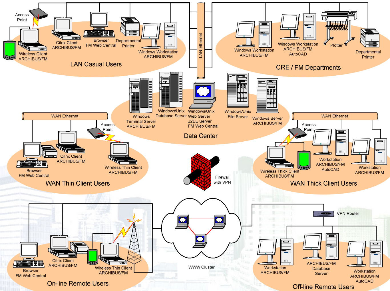
ARCHIBUS/FM Deployment Architecture
